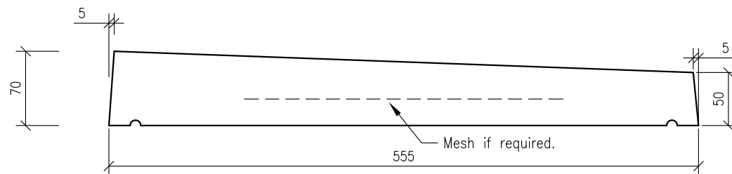
END VIEW.
