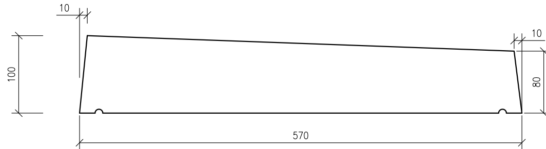
END VIEW.
