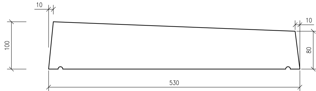
END VIEW.
