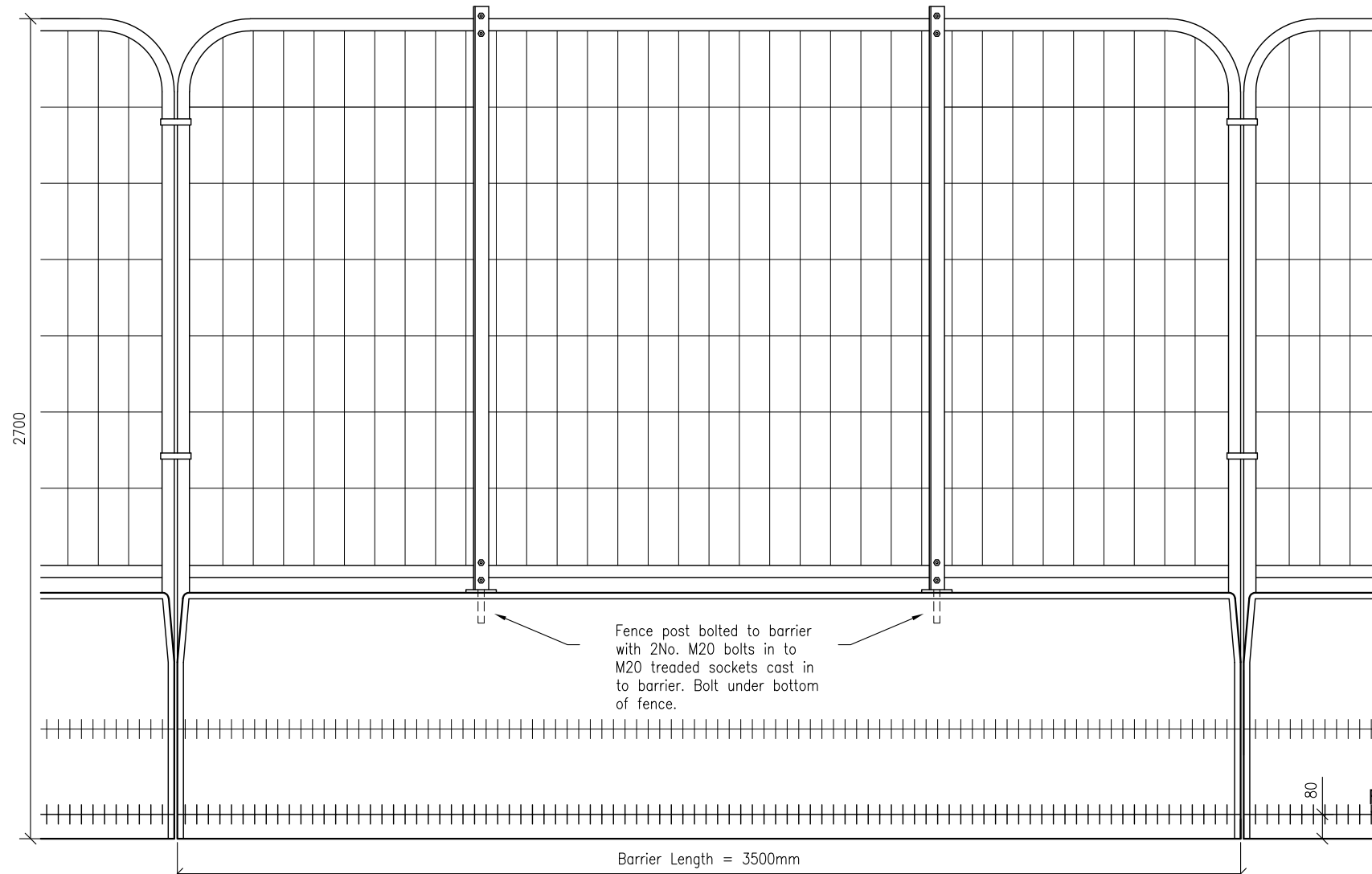
BACK ELEVATION (TO SHOW POSTS)
