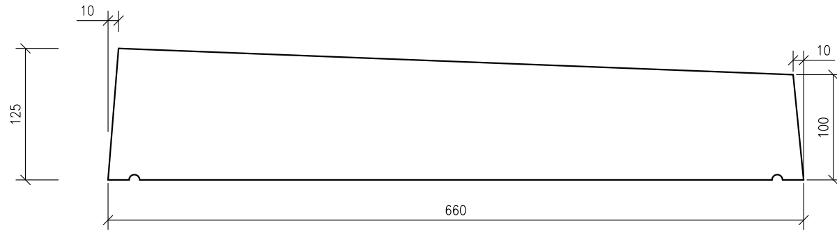
END VIEW.
