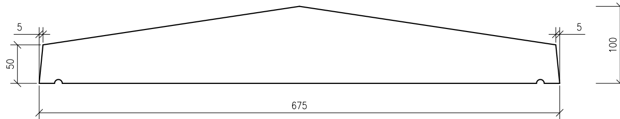
SECTION.
